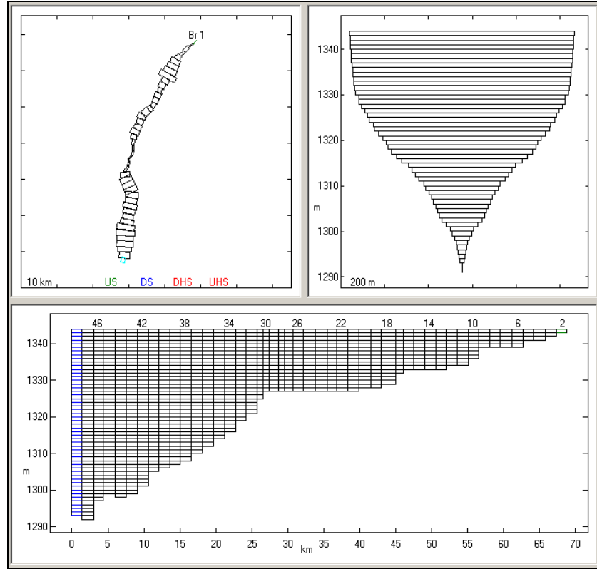
Figure 3.3 Elephant Butte bathymetry (clockwise: plan, front, and side views).
