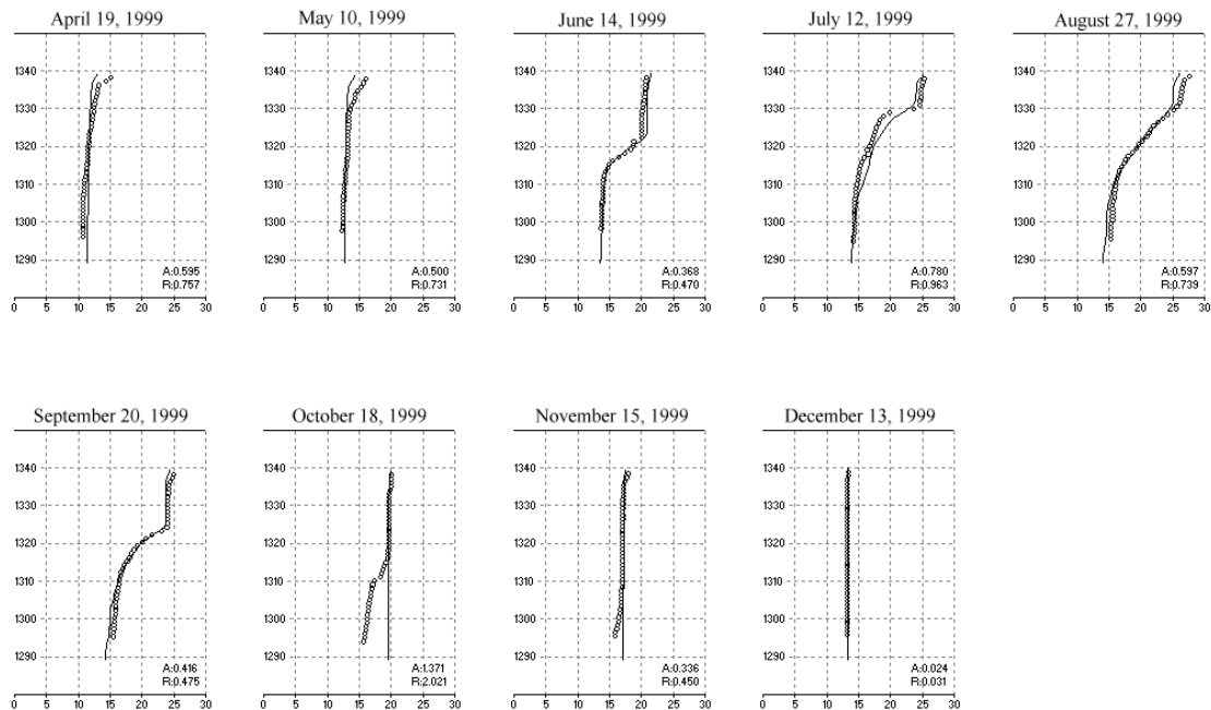
Figure 4.3 Calibrated Temperature Profile near the Dam for 1999.
