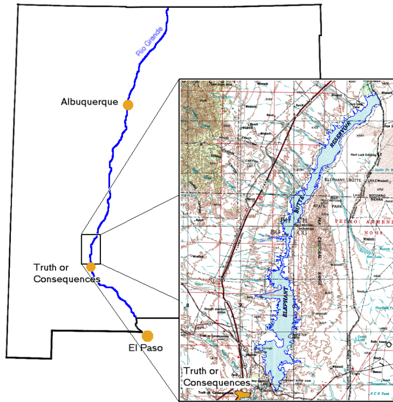
Figure 2.1 Map of Elephant Butte Reservoir.
