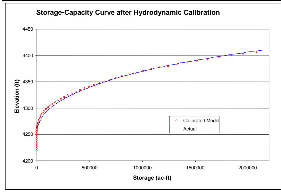
Figure 3.2 Results from calibration of bathymetry.
